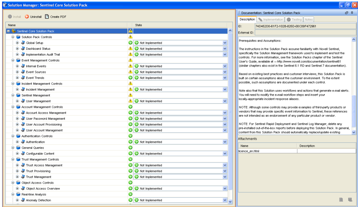
Figure 21-1 Solution Manager
