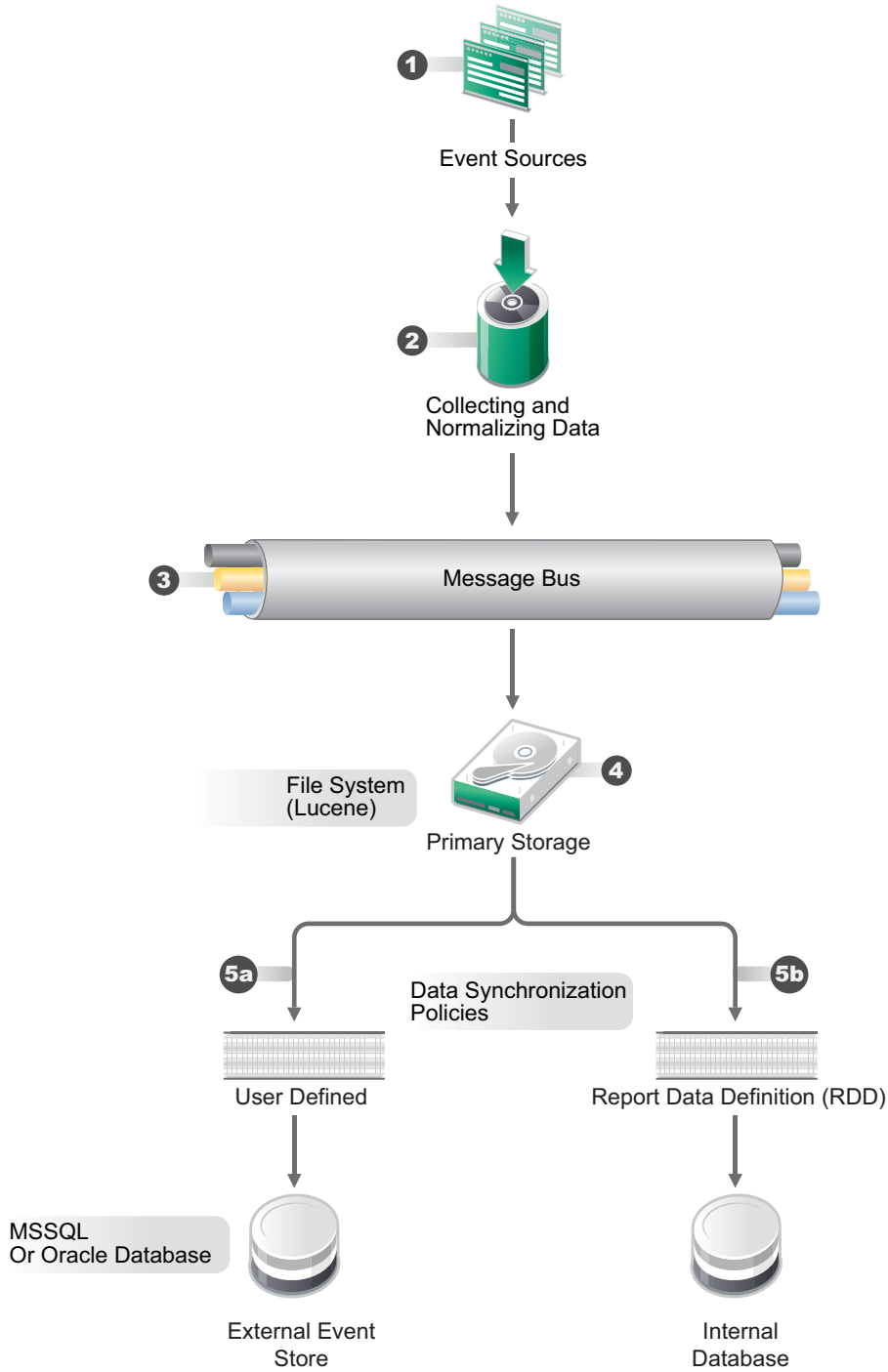
Figure 6-1 Data Synchronization
