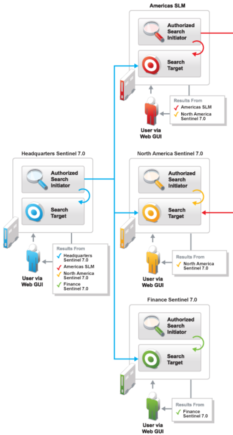
Figure 18-1 Distributed Search
