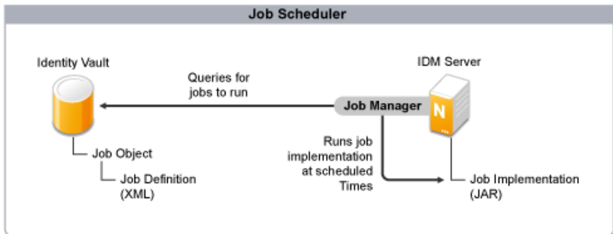
Figure 14-1 High-level View of the Job Scheduler Process
