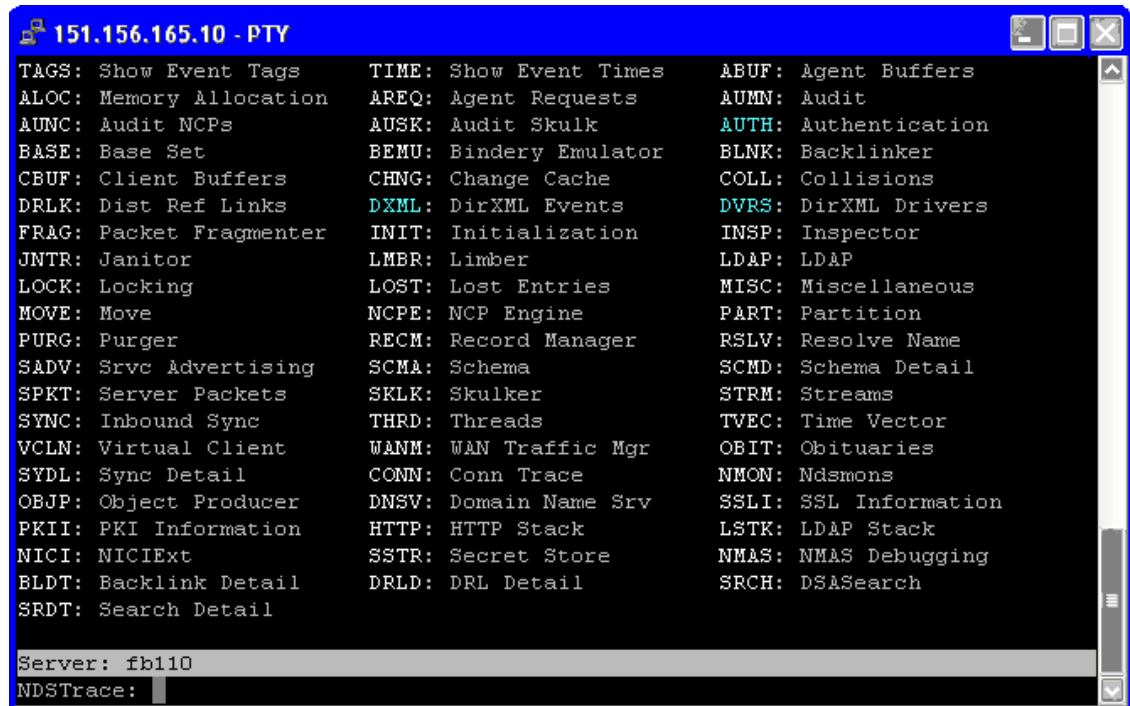
Figure A-5 DStTrace Commands
