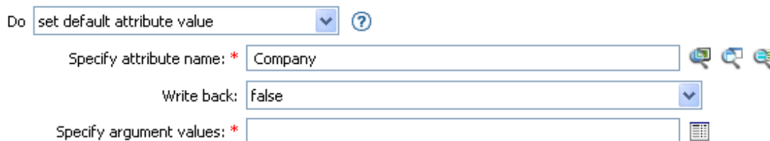
Figure 4-6 Set Default Attribute Value
