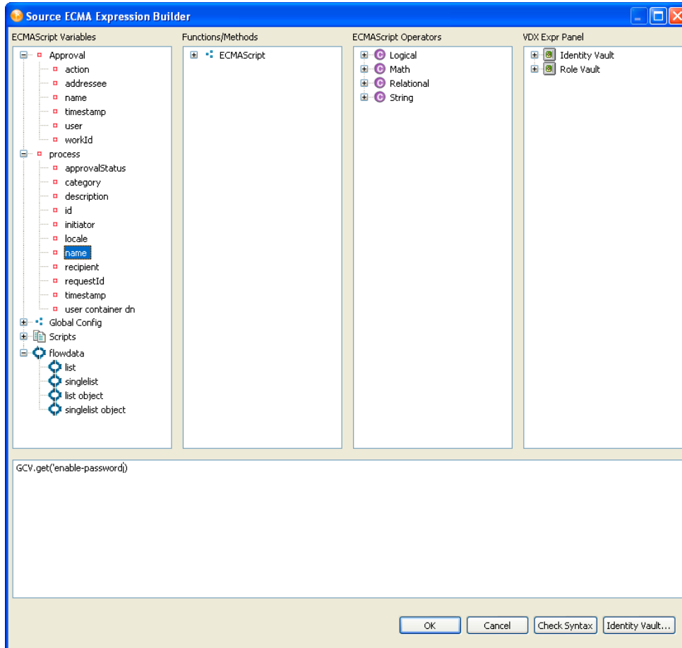
Figure 9-1 ECMA Expression Builder
