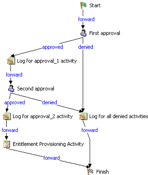
Figure 4-2 Sequential Workflow with Two Approvals
