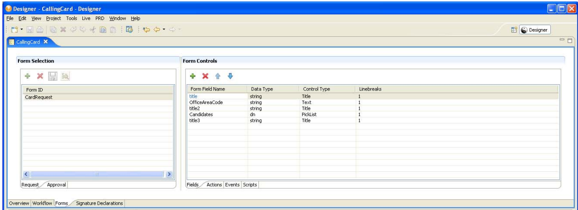
Figure 5-5 Forms Tab
