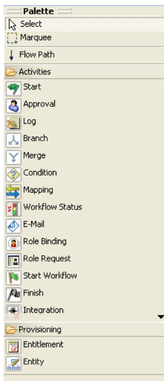
Figure 6-2 Workflow Palette
