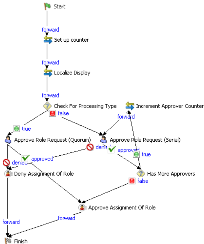
Figure 6-11 Default Resource Approval Workflow
