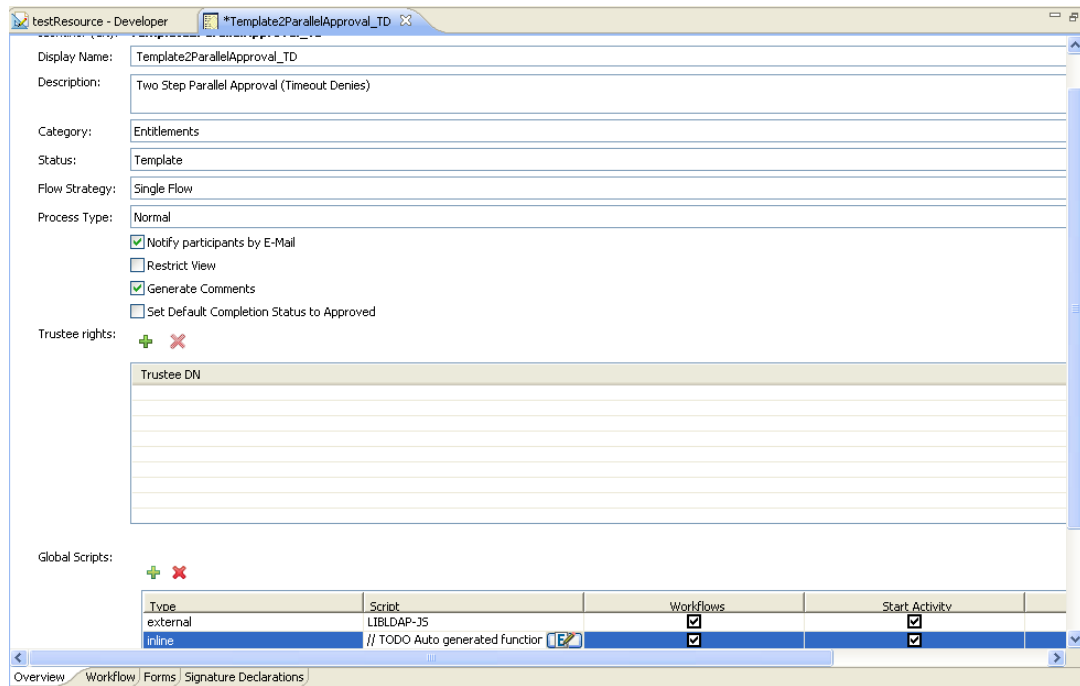
Figure 4-1 Overview Tab
