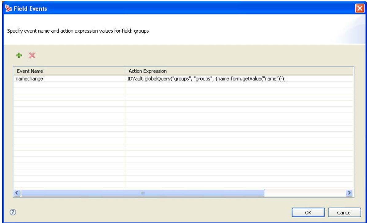
Figure 5-9 Custom Event Definition Example
