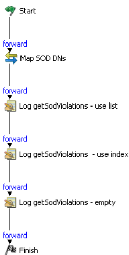
Figure 9-4 Sample Workflow for Retrieving SoDs
