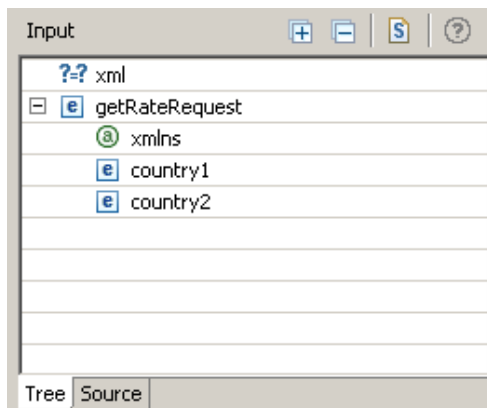
Figure 8-4 Input View
