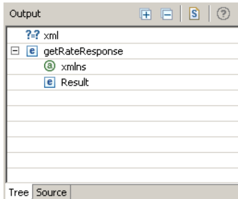
Figure 8-5 Output View
