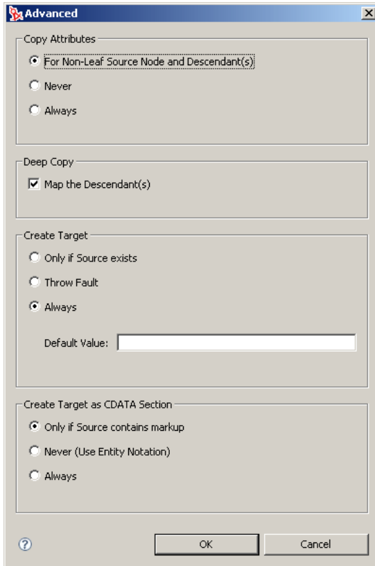
Figure 8-10 Advanced
