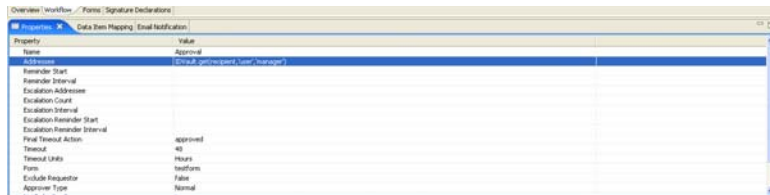
Figure 6-3 Workflow Views
