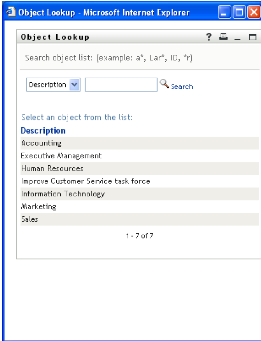
Figure 3-6 Object Lookup
