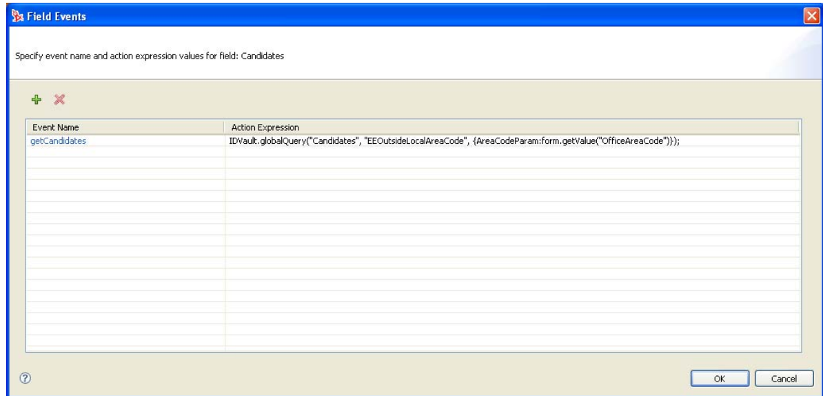
Figure 5-39 GetCandidates Event
