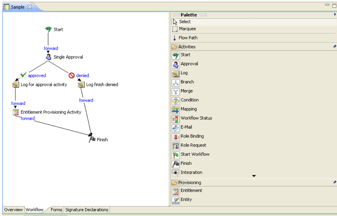
Figure 6-1 Workflow Page
