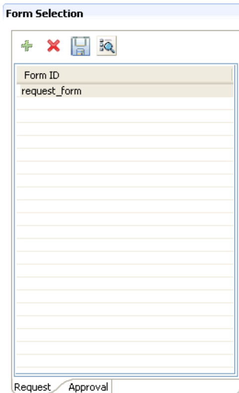
Figure 5-6 Form Selection
