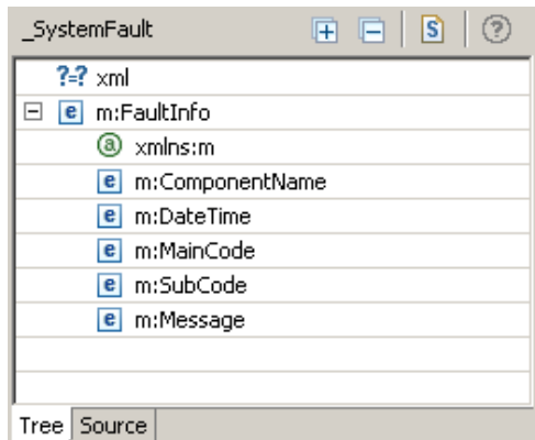
Figure 8-6 _SystemFault View
