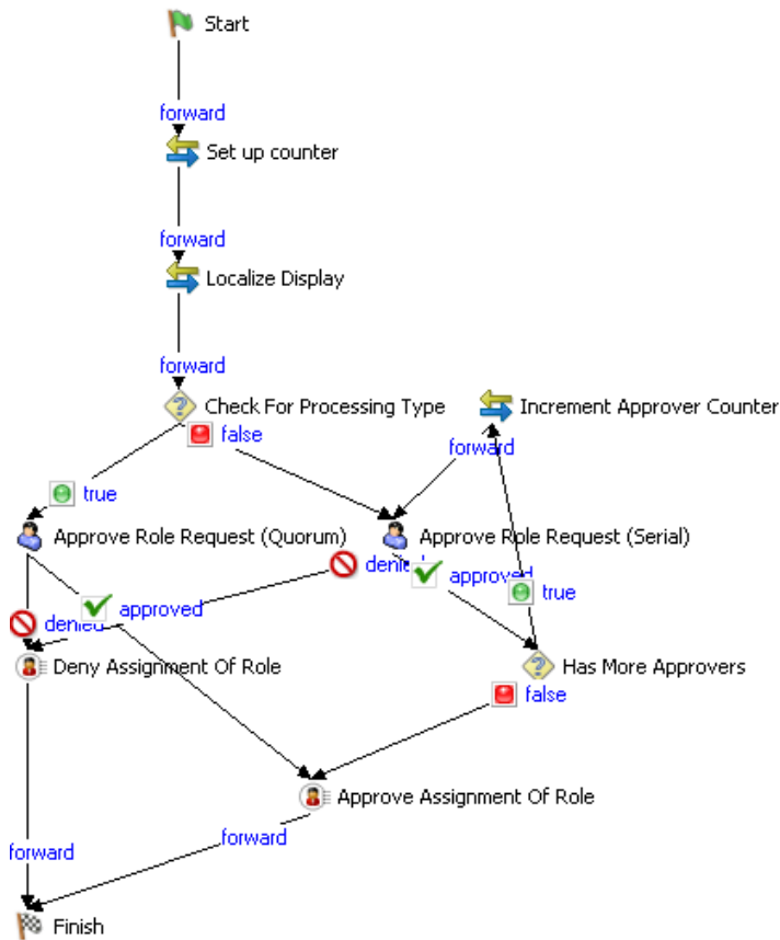
Figure 6-6 Default Role Approval Workflow
