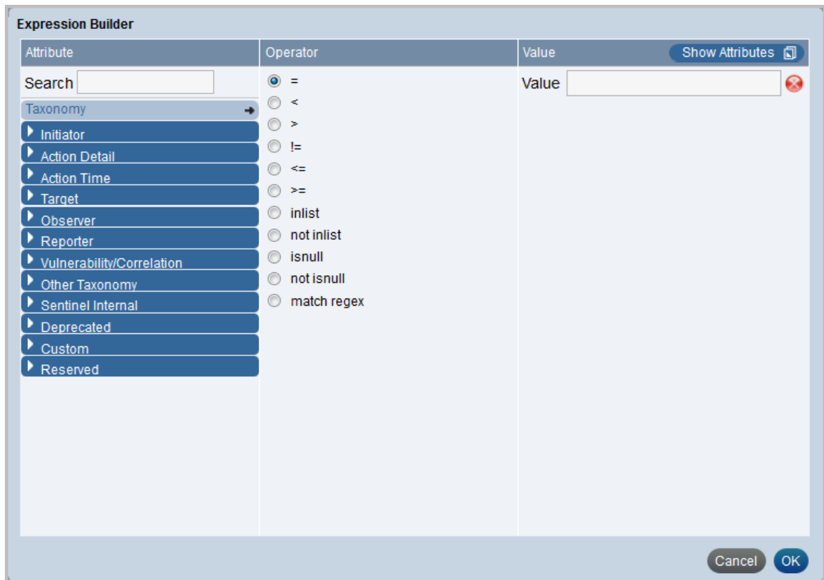
Figure 5-2 Expression Builder
