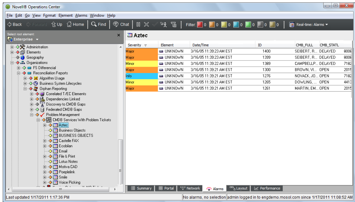
Figure 13-3 Alarms View
