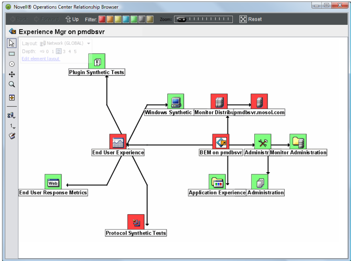
Figure 6-1 Relationship Browser
