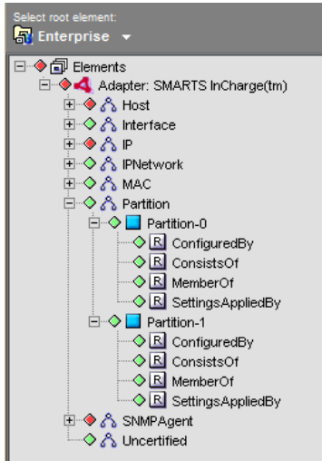
Figure 2-6 Explorer Pane: InCharge objects are listed under the adapter element
