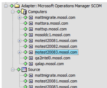
Figure 2-19 Event Integration: Incoming events are grouped by Computer ID and Source
