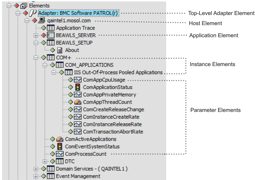
Figure 2-1 PATROL hosts, applications, instances and parameters display under the PATROL adapter in the Explorer pane
