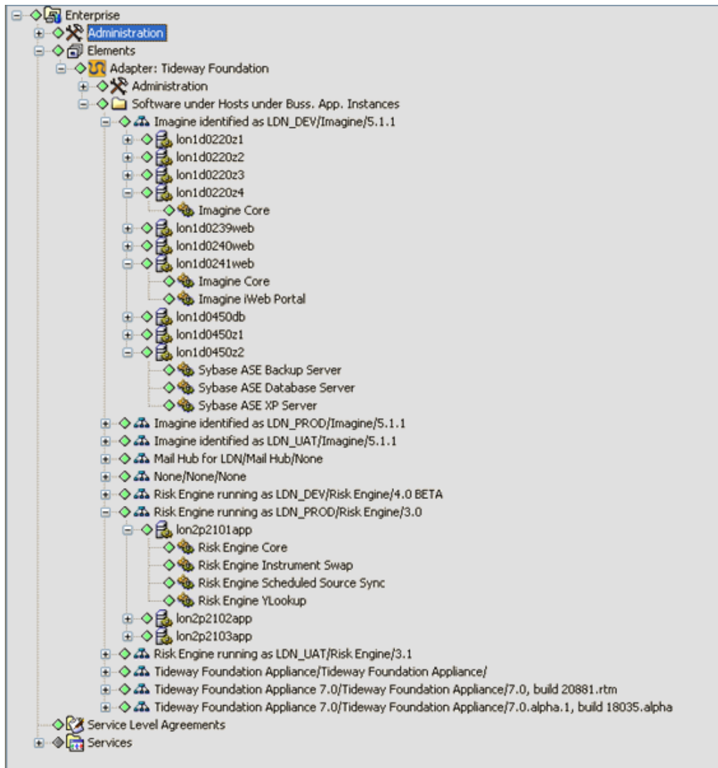
Figure 3-5 Operations Center Console Showing Software Instances
