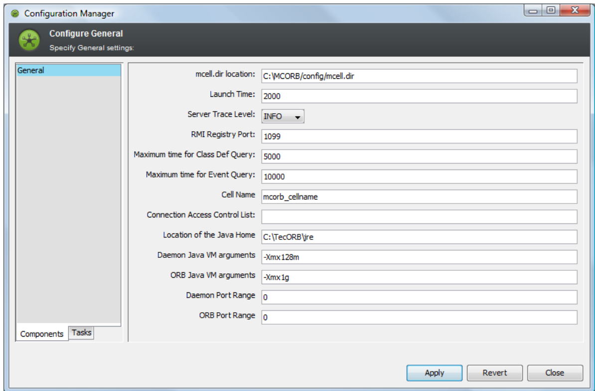
Figure 10-1 Configuration Manager Dialog Box for MCOB
