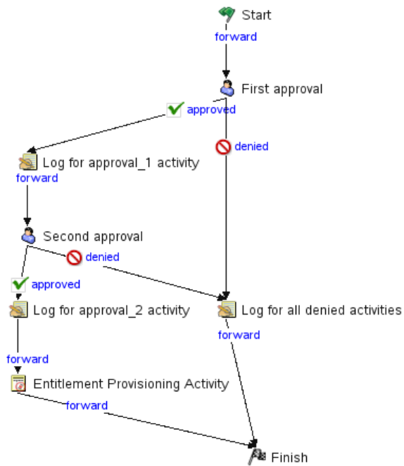
Figure 4-1 Sequential Workflow with Two Approvals
