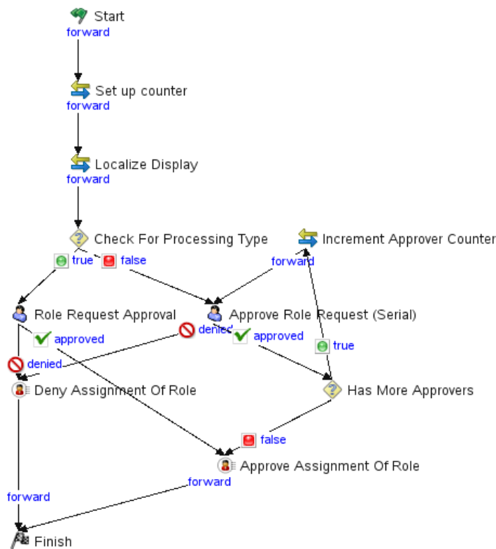
Figure 6-11 Default Resource Approval Workflow
