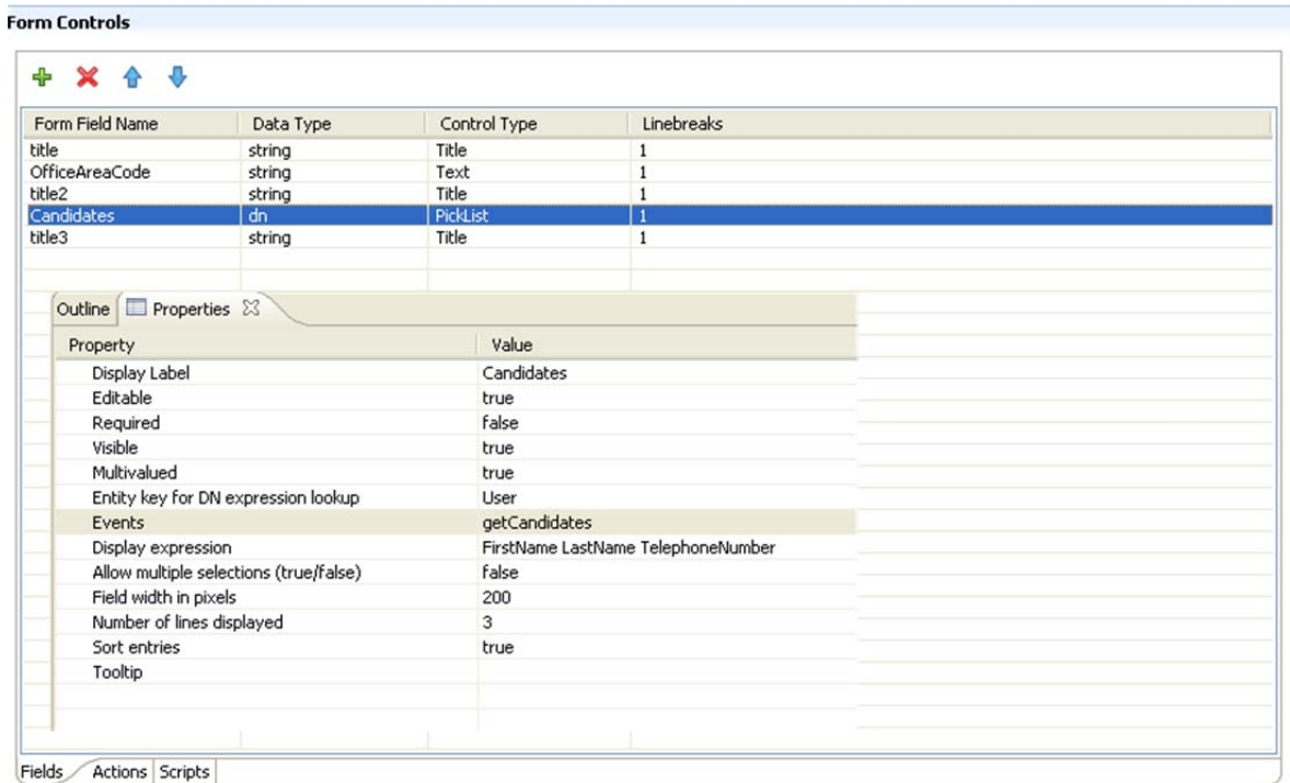
Figure 5-39 Candidates PickList Properties
