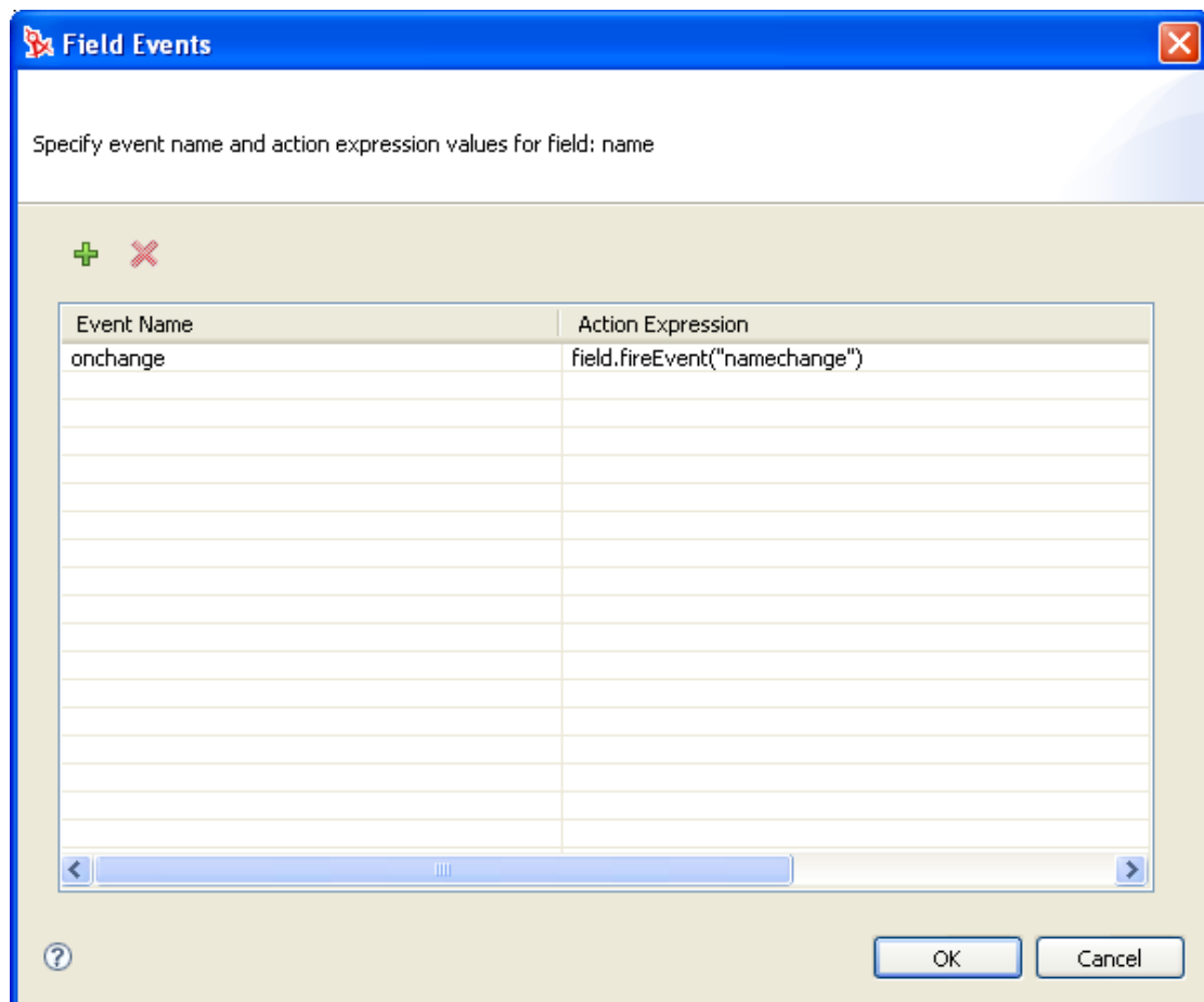
Figure 5-10 Sample field.FireEvent() Method
