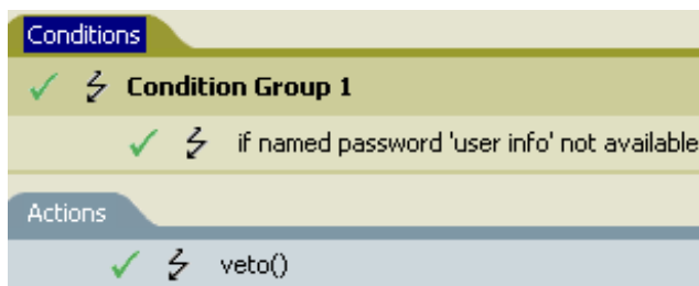
Figure 10-1 A Policy Using Named Passwords
