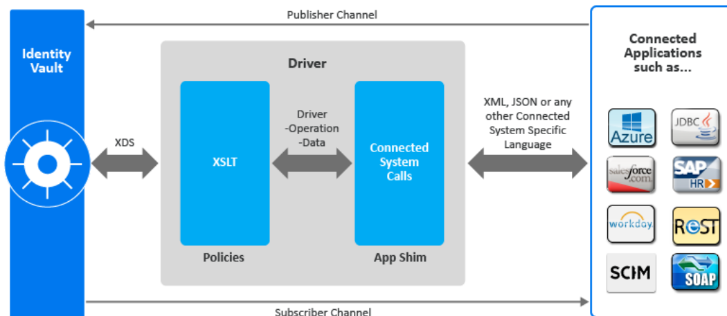
Figure 1-1 Driver Dataflow
