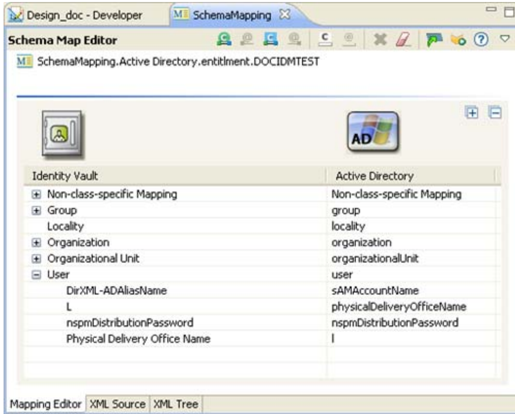
Figure 6-1 The Schema Map Editor
