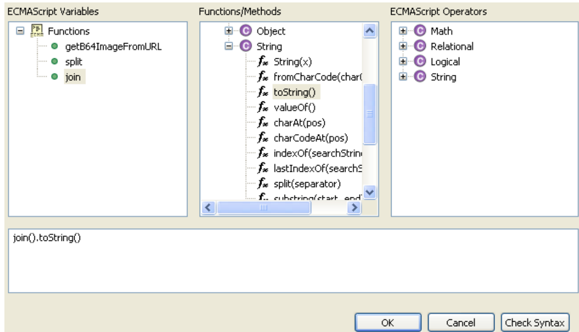
Figure 11-3 Expression Builder Example
