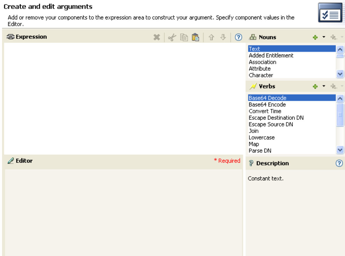
Figure 3-2 Argument Builder
