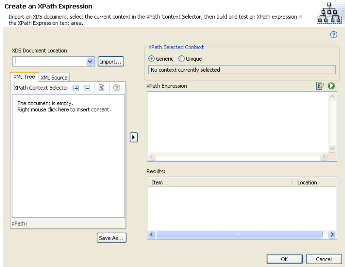
Figure 5-1 XPath Builder
