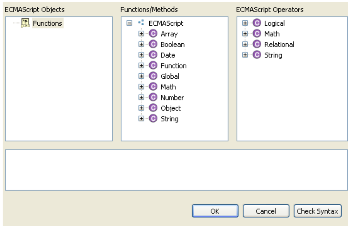
Figure 11-2 Expression Builder
