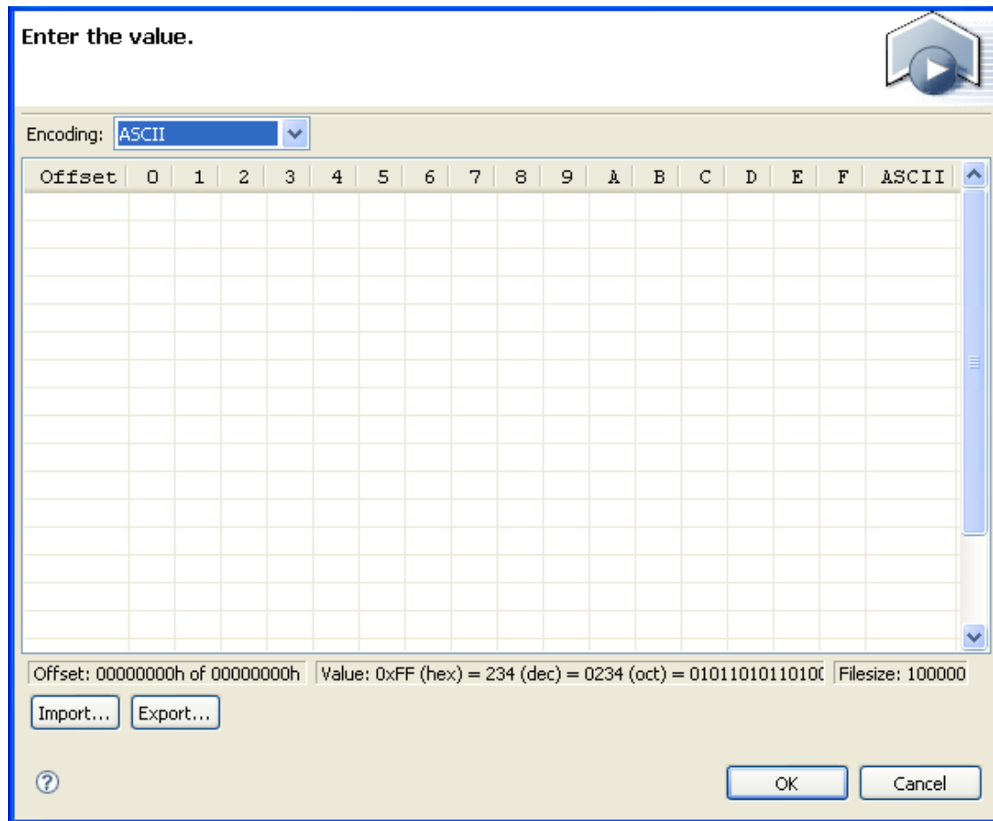
Figure 9-6 Hex Editor
