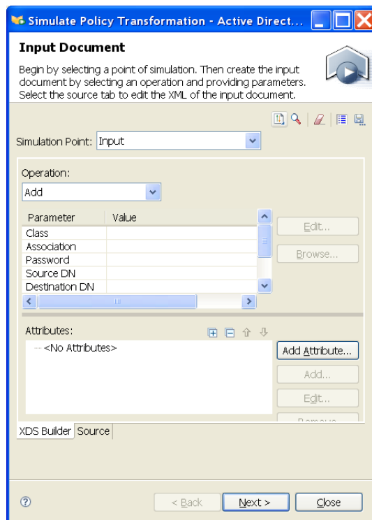
Figure 9-1 XDS Builder
