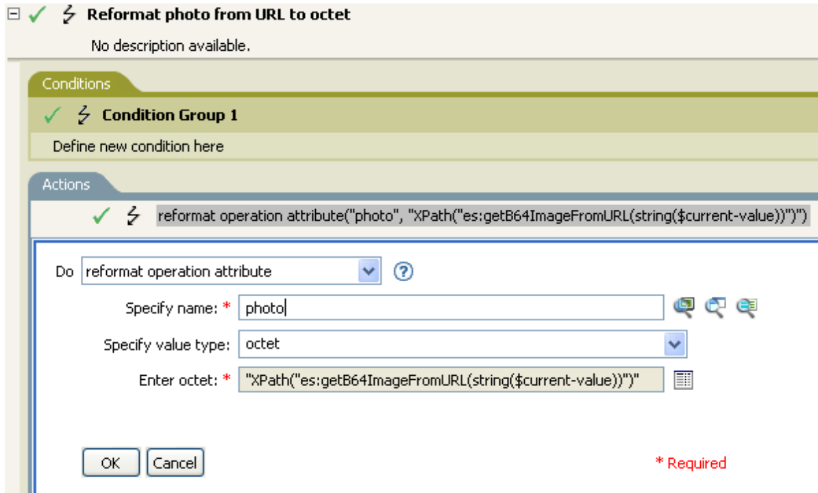
Figure 11-8 Reformat Photo Example
