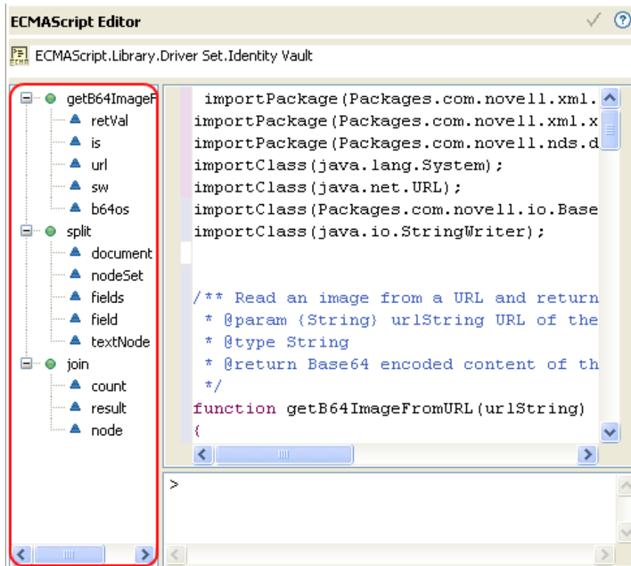
Figure 11-4 Functions and Variables
