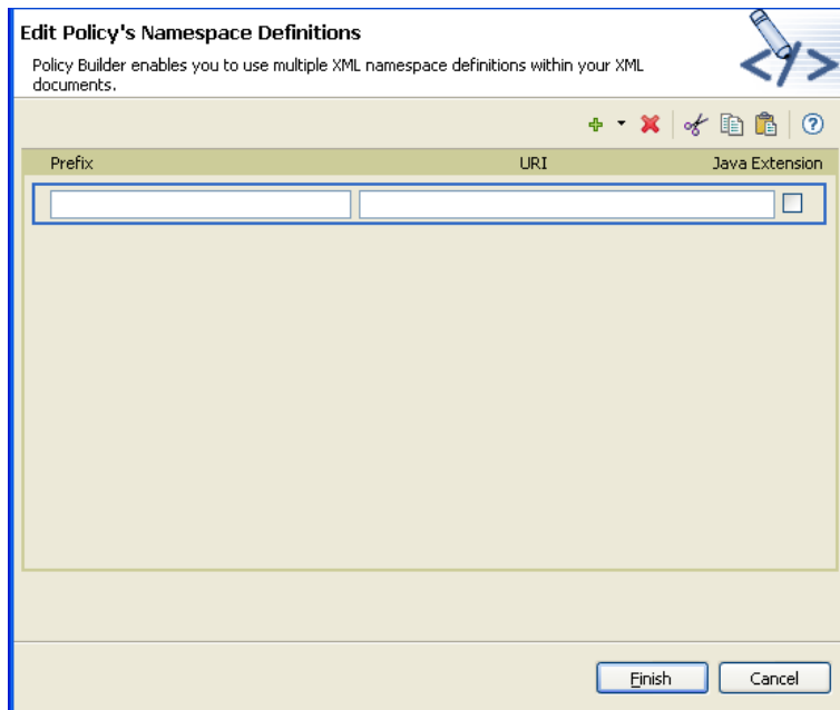
Figure 16-8 Namespace Editor
