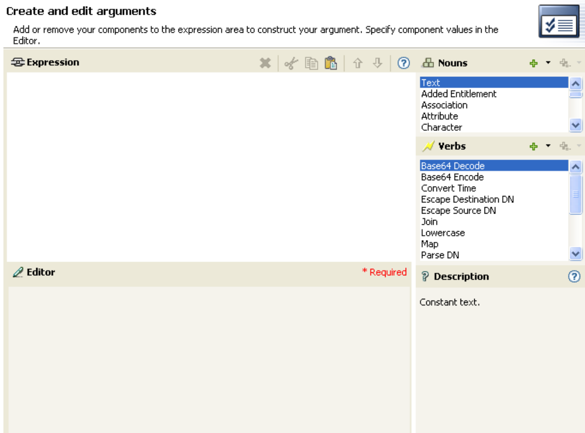
Figure 4-3 Argument Builder
