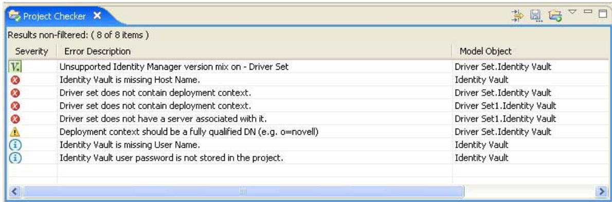
Figure 4-6 Project Checker
