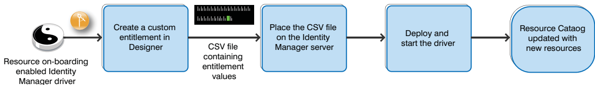
Figure 19-2 Custom Entitlements Creation
