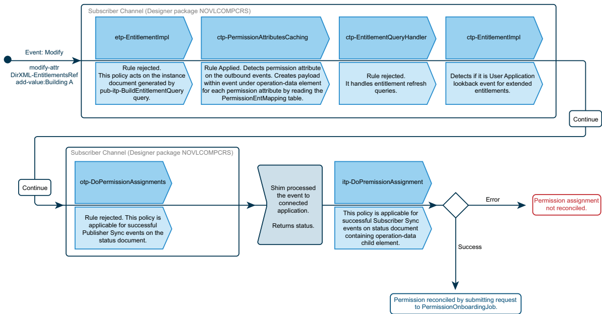
Figure 19-4 Subscriber Channel Identity Vault Attribute Permission Assignment Sequence
