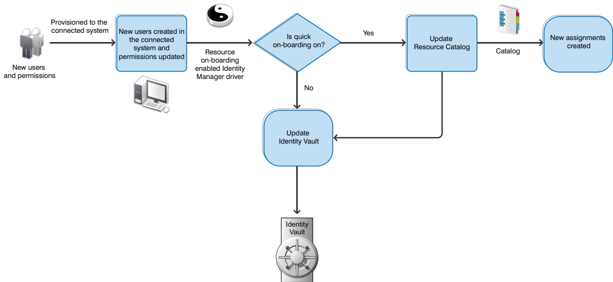
Figure 19-1 Flow of New Users and Permission Assignments
