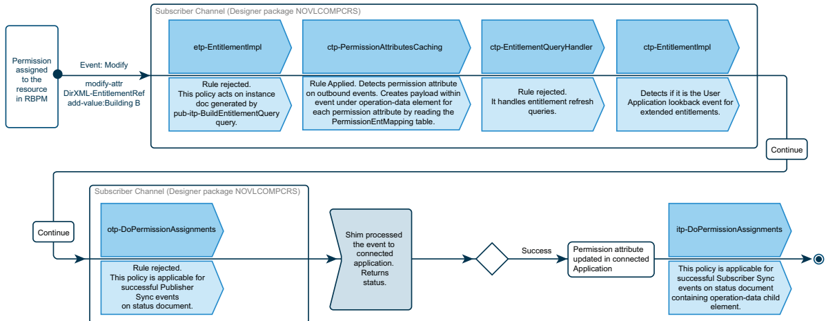
Figure 19-5 Subscriber RBPM Permission Assignment Sequence
