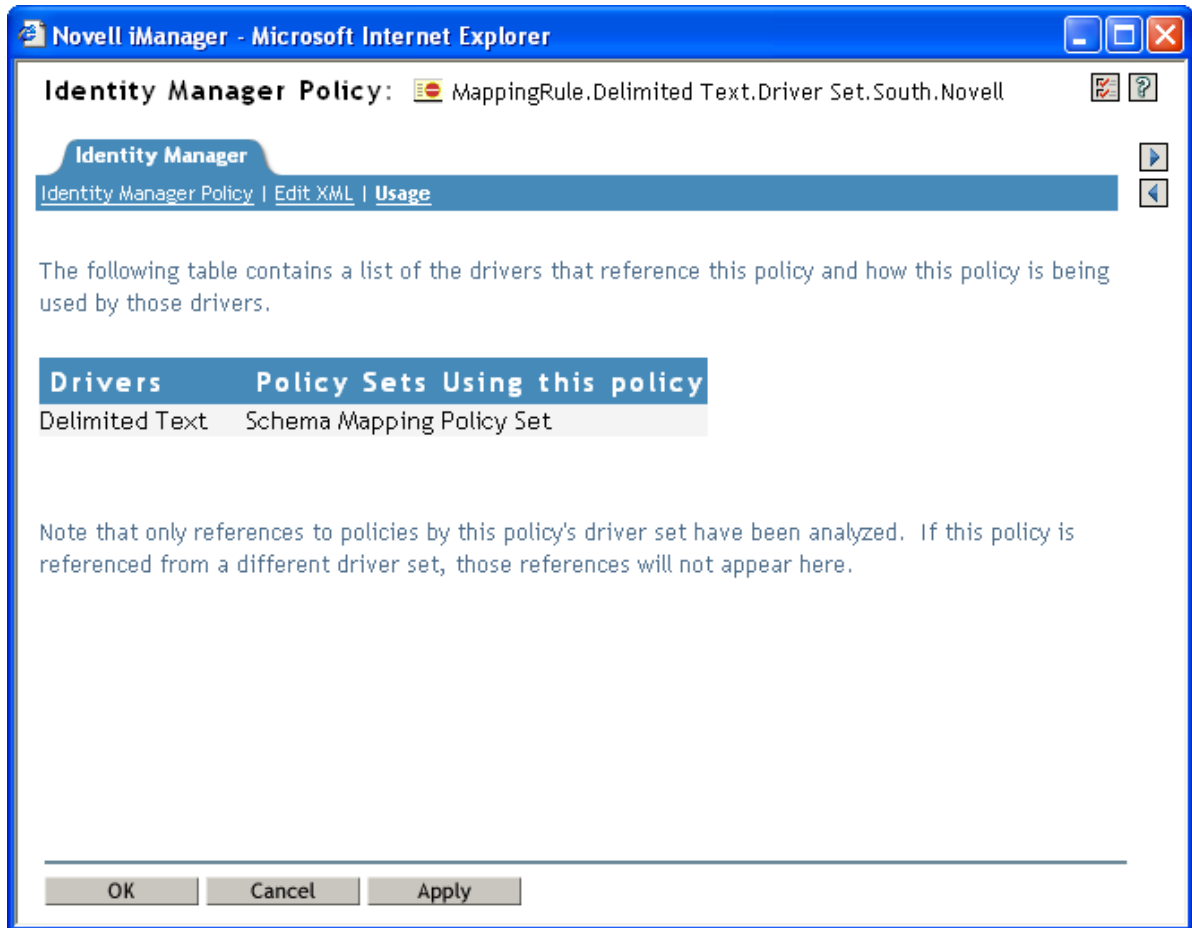
Figure 4-2 Usage
