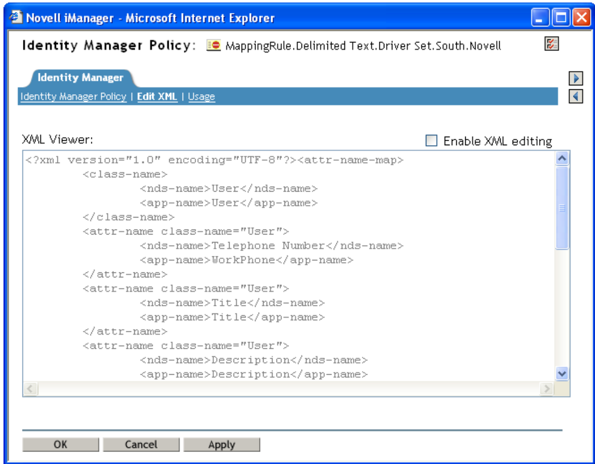
Figure 4-1 Edit XML
