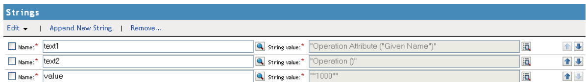
Figure 3-6 String Builder
