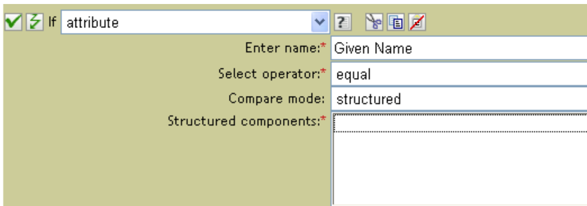
Figure 3-8 Structured Option
