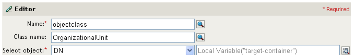
Figure 6-1 Create Container
