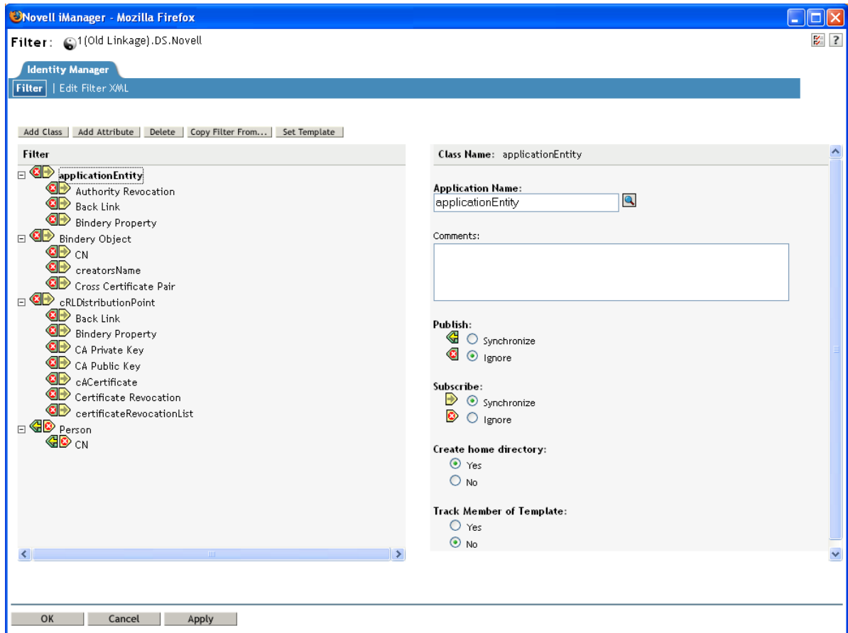
Figure 5-1 Filter Editor
