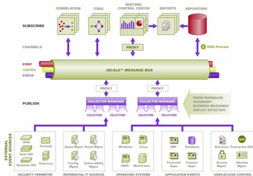
Figure 7-1 Sentinel Architecture
