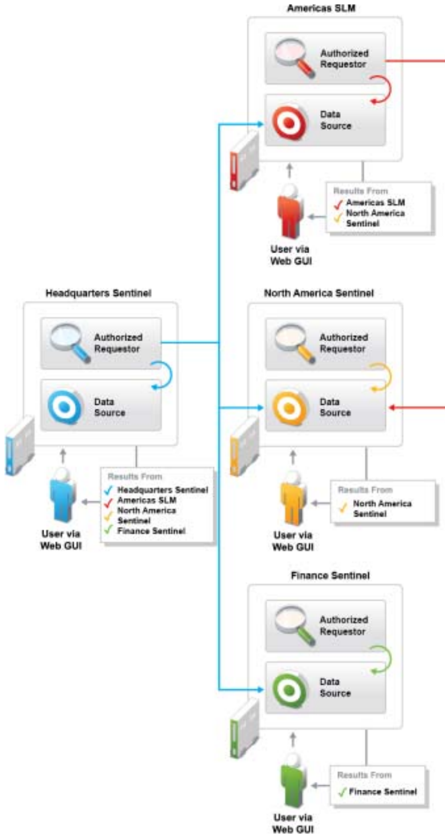
Figure 21-1 Data Federation
