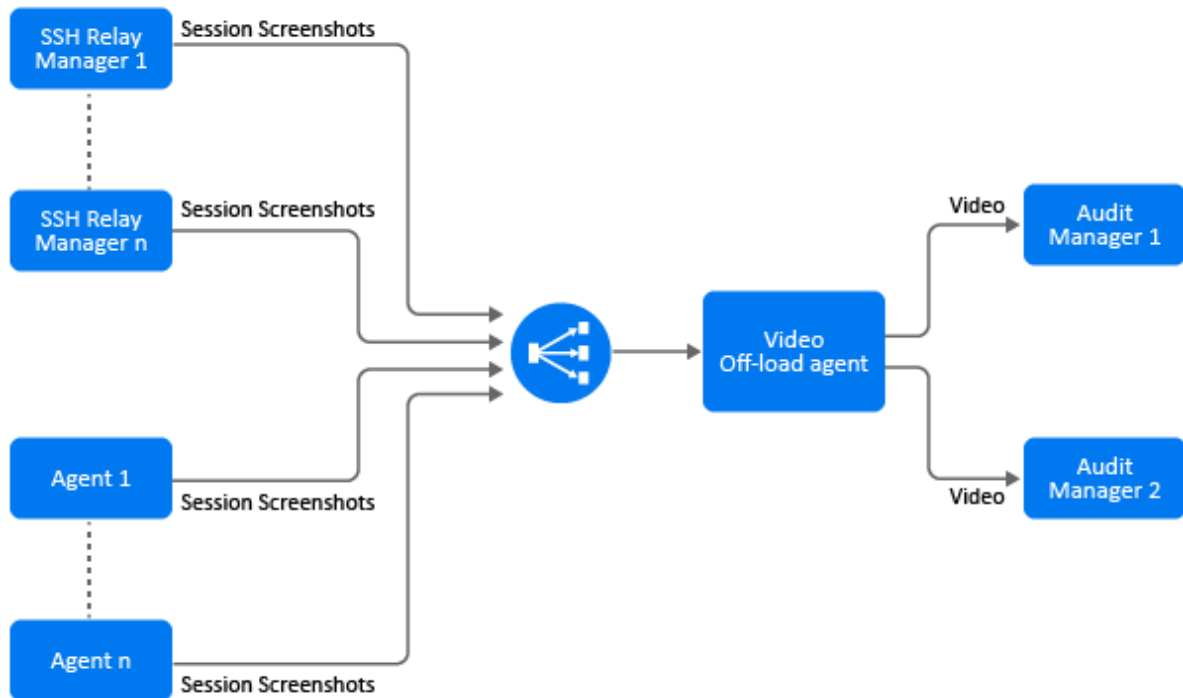
Figure 8-2 The following illustrations explains the flow of the video generation process with multiple audit managers:
