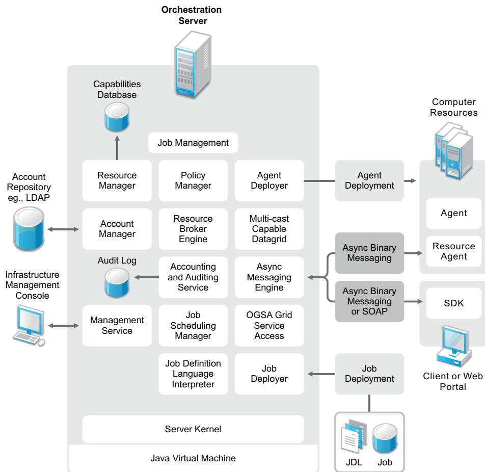
Figure 5-2 Cloud Manager Orchestration Grid Architecture
