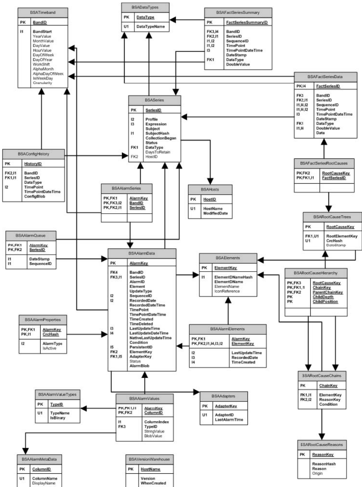
Figure 3-1 Table Relationships
