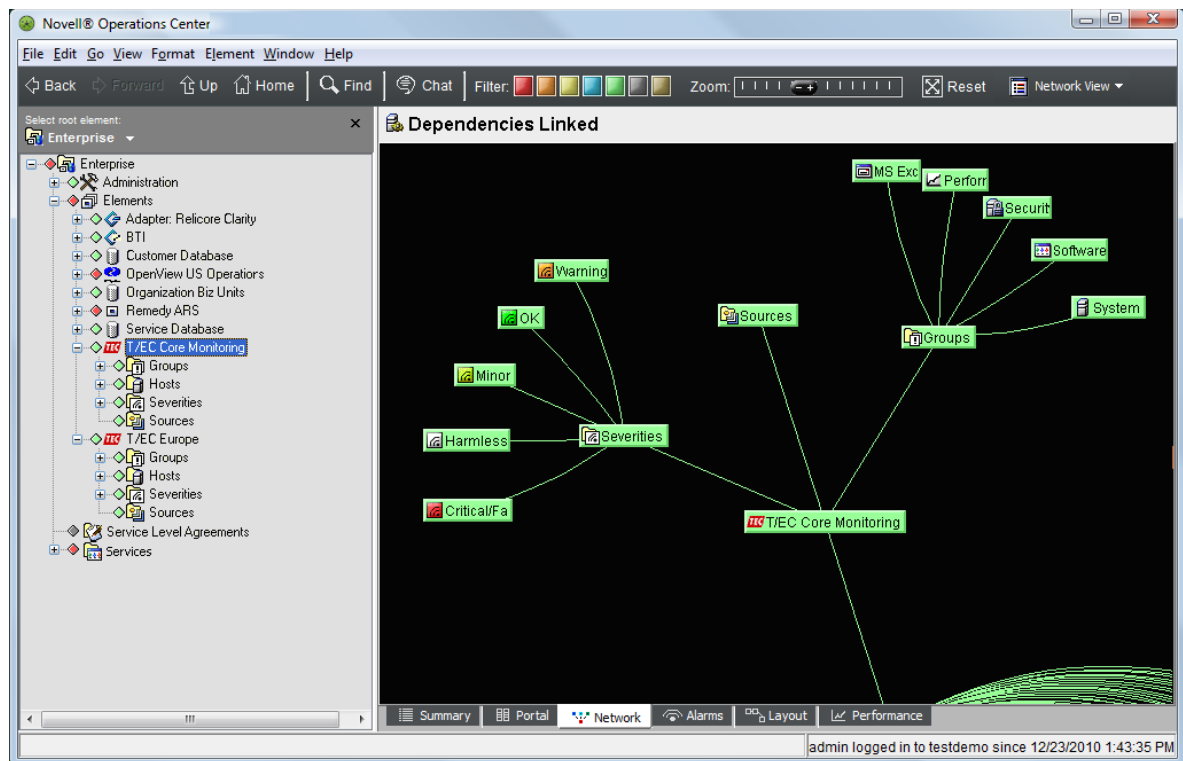
Figure 10-1 Network View
