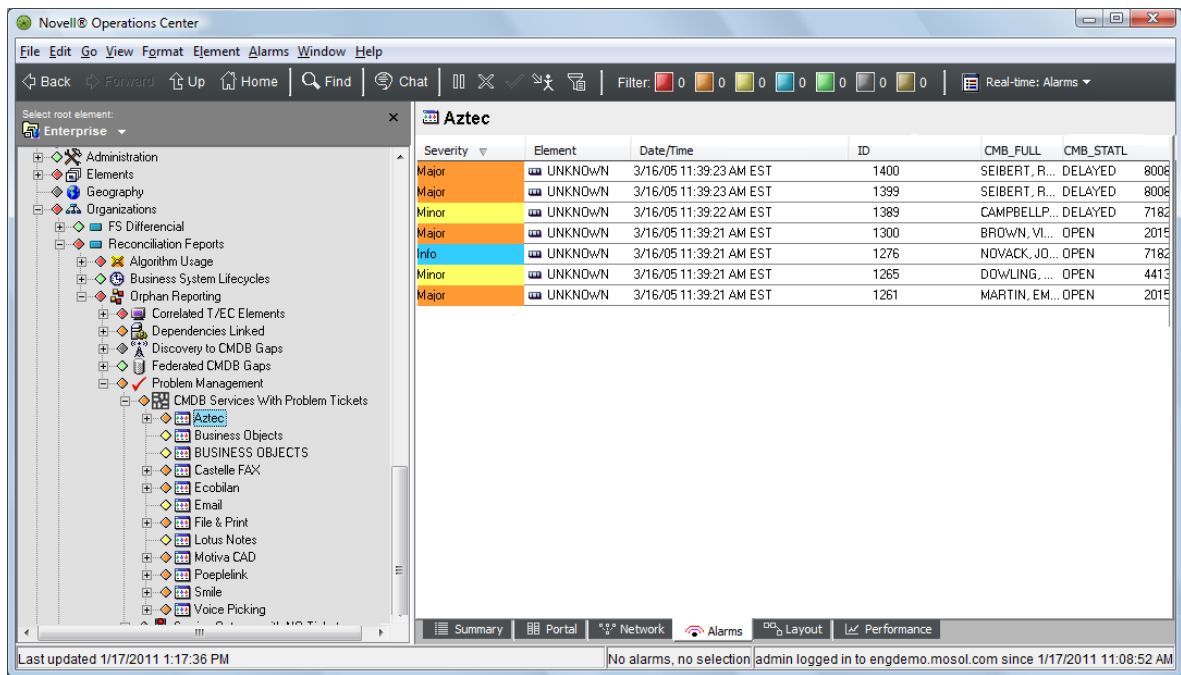
Figure 13-3 Alarms View
