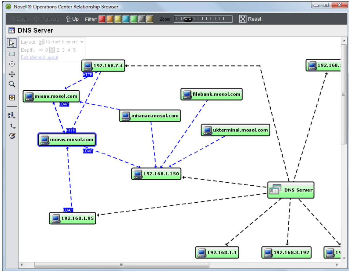
Figure 6-2 Relationship browser
