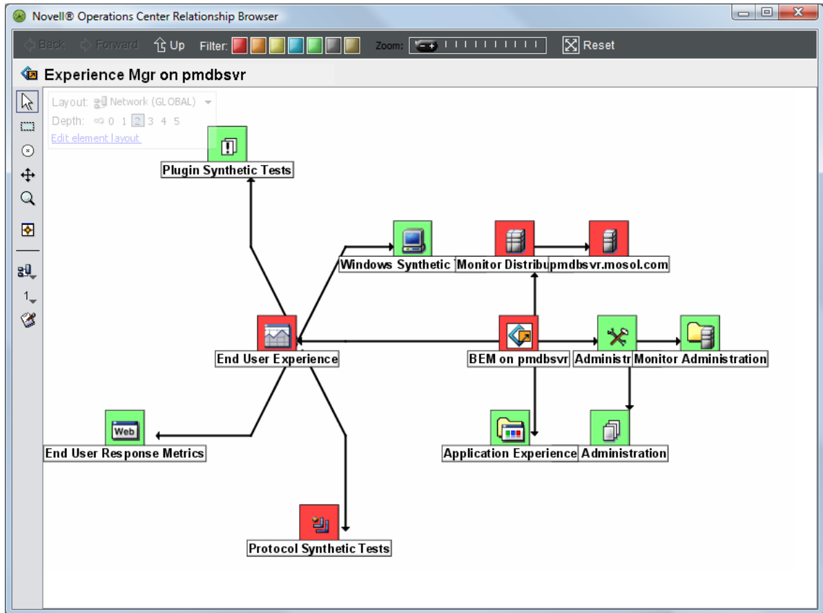
Figure 6-1 Relationship Browser
