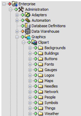
Figure 4-1 Clipart Hierarchy
