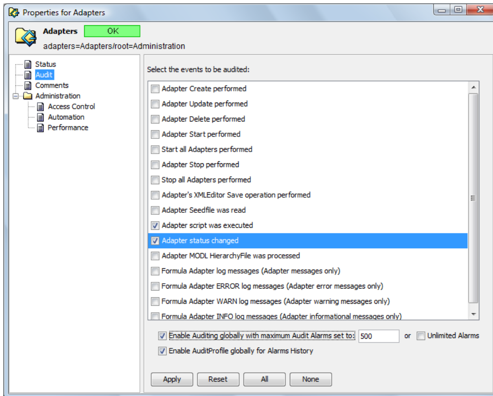
Figure 6-2 Adapter Audit Properties
