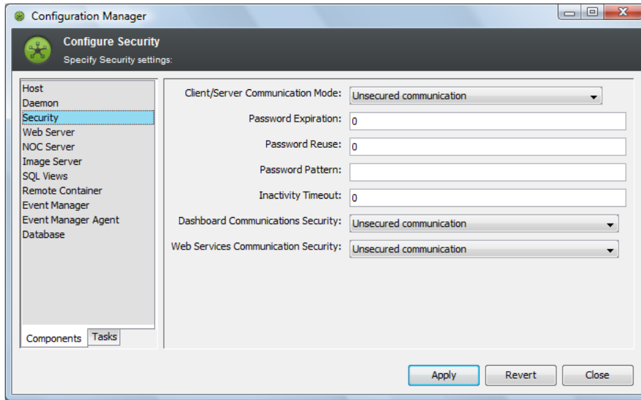
Figure 5-1 Operations Center Configuration Manager Security Pane
