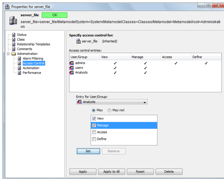
Figure 4-8 Class Element Access Control Property Page
