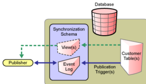
Figure 1-5 Direct Synchronization on the Publisher Channel
