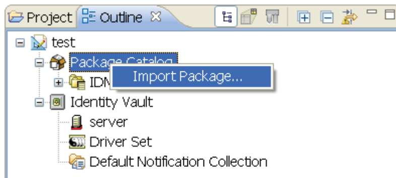
Figure 3-1 Import Package
