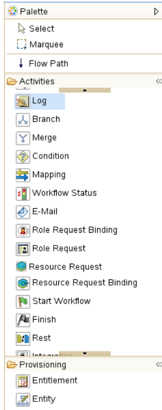
Figure 6-2 Workflow Palette
