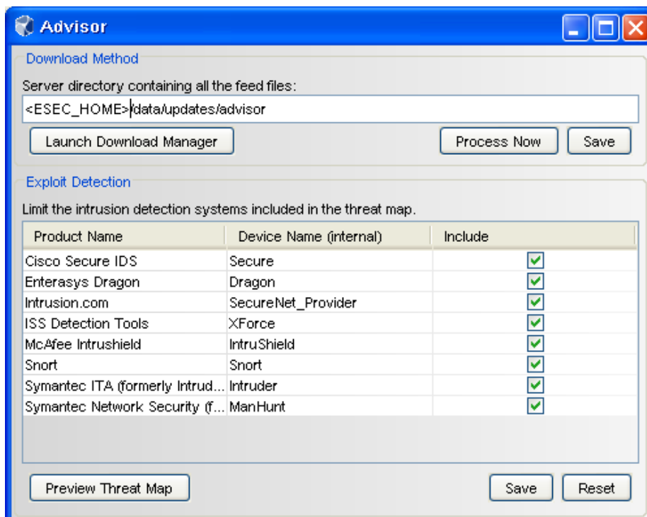
Figure 19-1 Advisor Window
