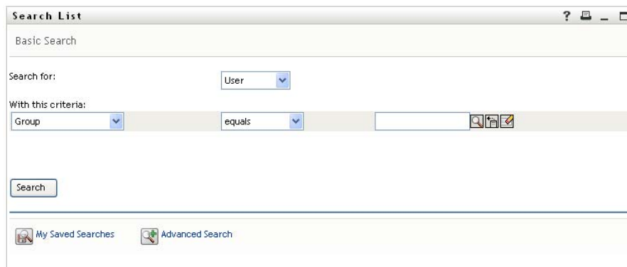
Figure 3-5 Search Criteria
