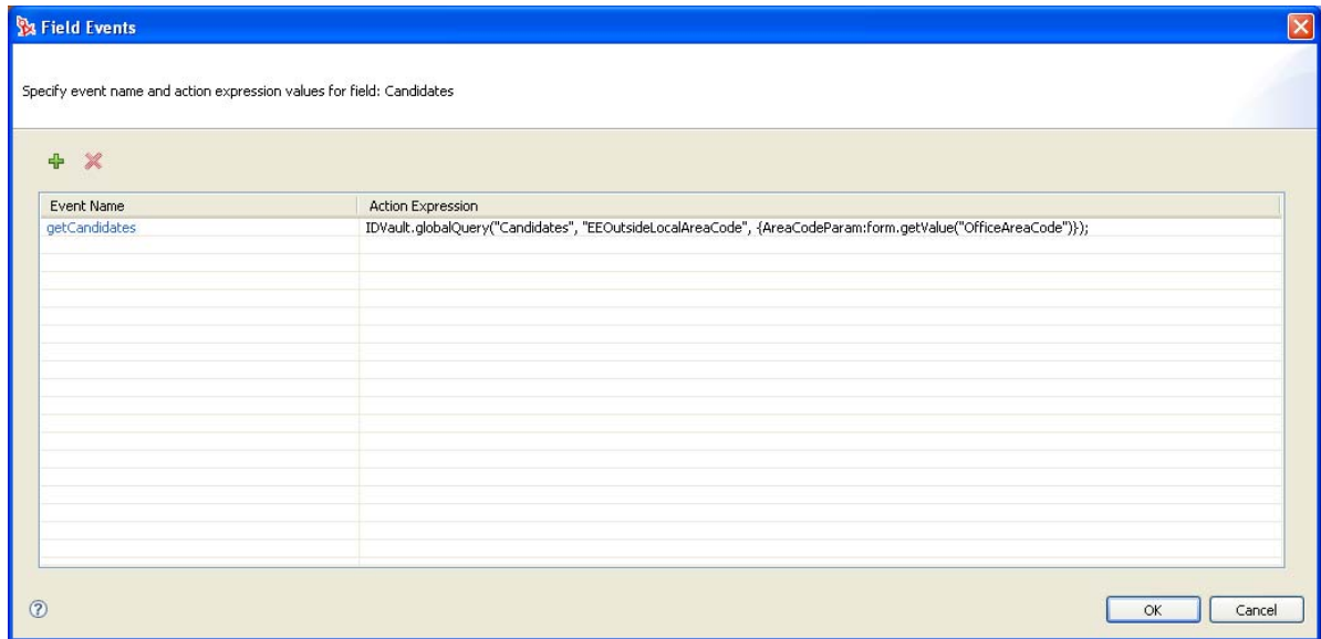
Figure 5-31 GetCandidates Event
