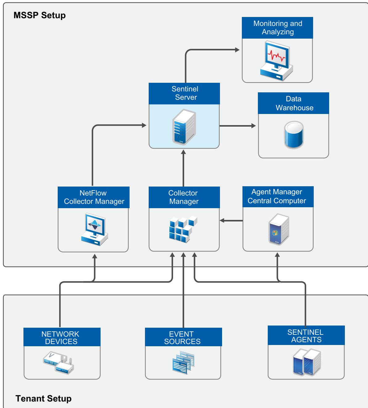
Figure 39-3 Full SaaS or Cloud Model
